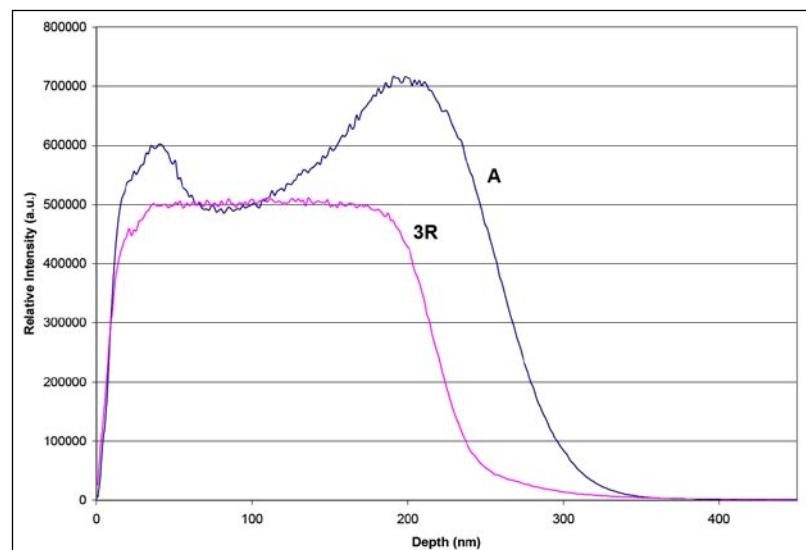
Figure 4 – Comparison of C profiles for unreflowed (A) and reflowed (3R) OSP layers obtained by Dynamic SIMS
