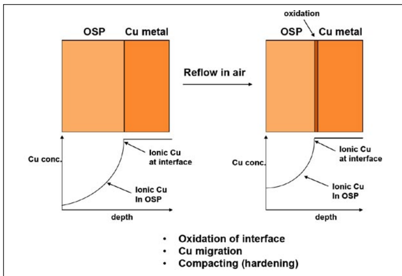
Figure 5 – Suggested changes within OSP coating during heat treatments
