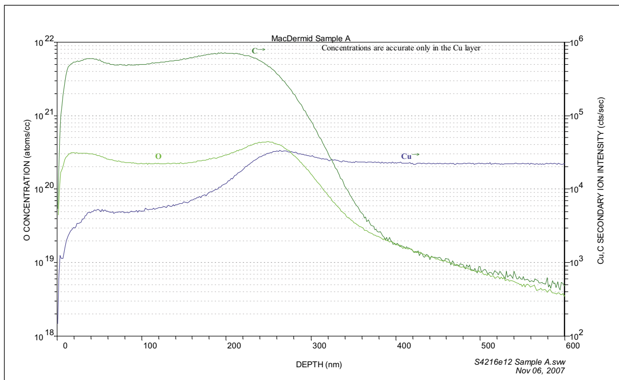
Figure 1 – Profiles of C, O and Cu concentrations within as coated OSP layer obtained by dynamic SIMS
