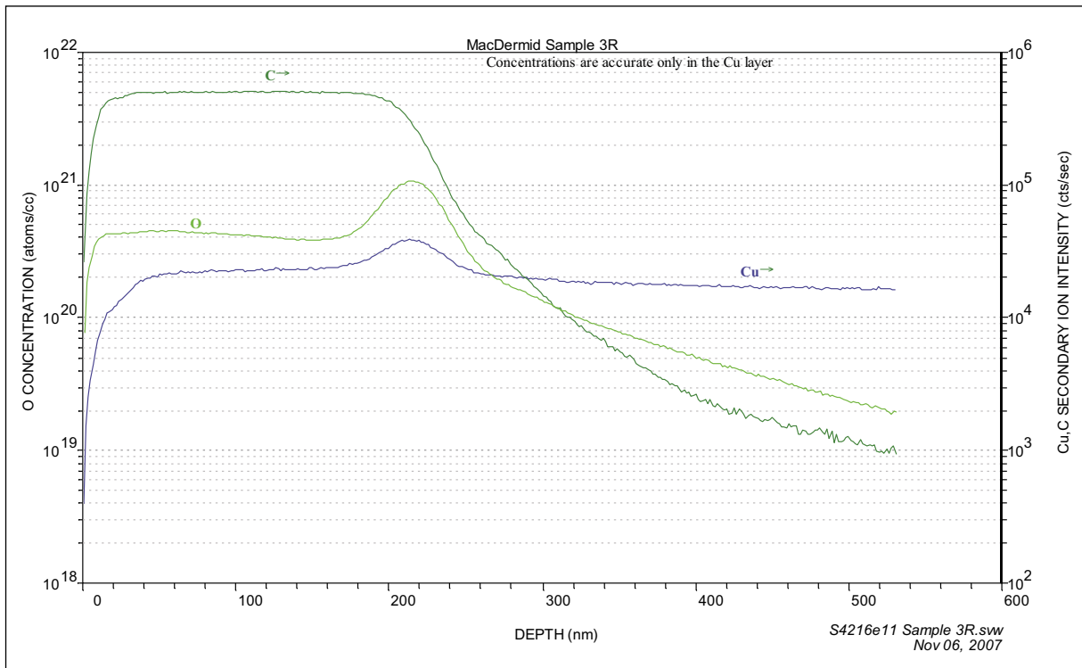
Figure 3 – Profiles of C, O and Cu concentrations within OSP layer reflowed three times obtained by Dynamic SIMS
