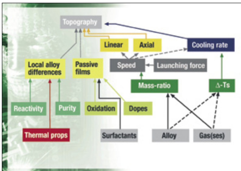
Figure 3 - A map of some of the parameters impacting the topography of solder particles. DOEs may demonstrate which are the most significant
