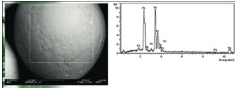
Figure 7a (left) - EDX-Image of a SAC-solder particle with Sn95.5/Ag4.0/Cu0.5. The analysis (Figure 7b - right) however results in a percentage [w/w] distribution on the surface of Sn94.6/ Ag4.4/Cu1.0
