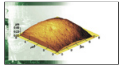
Figure 6 - A 3D-image of a surface of 64 \mu\text{m}^2 of a Sn95.5/Ag4.0/Cu0.5 solder particle generated by atomic force microscopy (AFM). The average nano-surface roughness (Ra) is 9.2 nm
