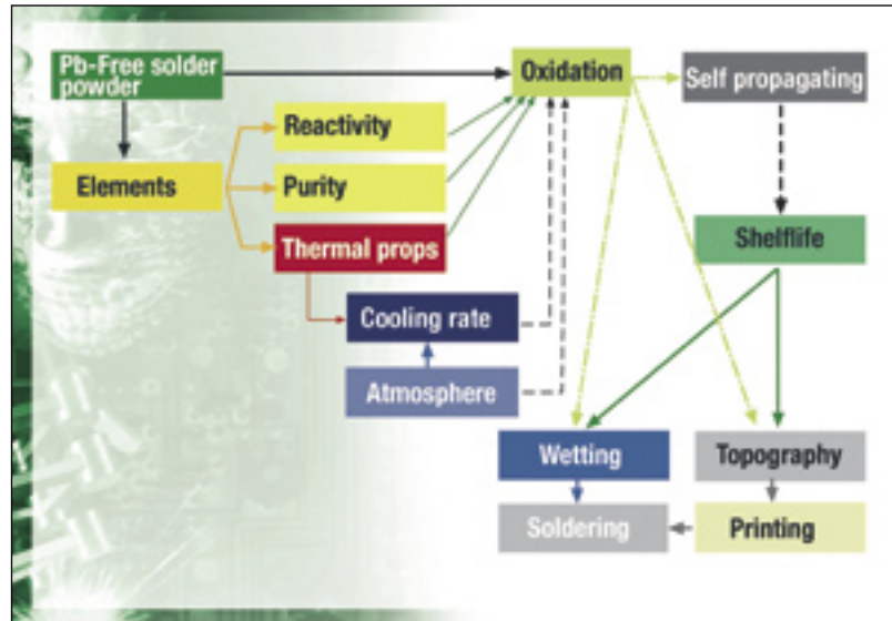
Figure 2 - A mind map approach to the interactions that should be addressed when designing for the production of Pb-free soldering paste
